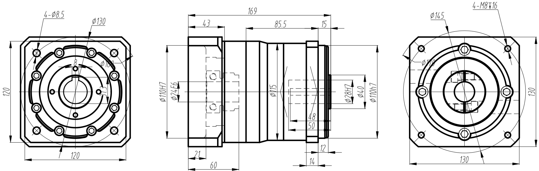
标准轴 Standard output shaft
